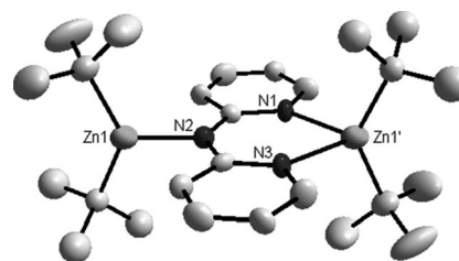
Figure 4. Anion of the solvent-separated ion pair structure of 4 [26] with thermal ellipsoids at 50% probability level. Hydrogen atoms and disordered components omitted for clarity. The anionic moiety of 5 is effectively identical.
