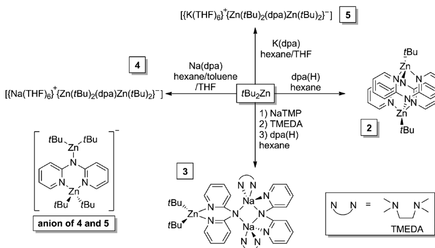
Scheme 1. Synthesis of the neutral zinc dimer 2 , sodium zincate 3 , sodium zinczincate 4 , and potassium zinczincate 5 .
